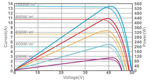
I-V characteristics at different irradiances
